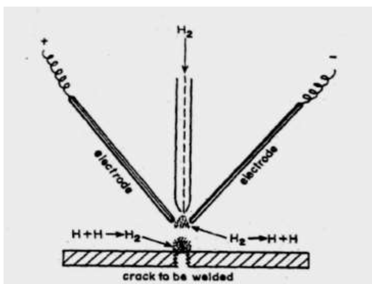
Fig. 4.1 Atomic Hydrogen Welding Torch
