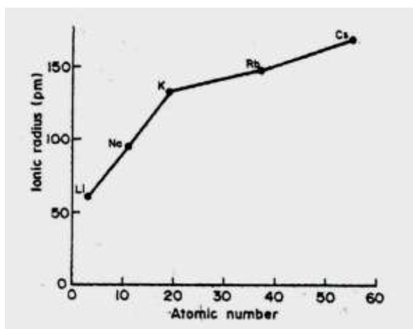
Fig. 2.2 Trend in Ionic Radii of Group 1 Elements
