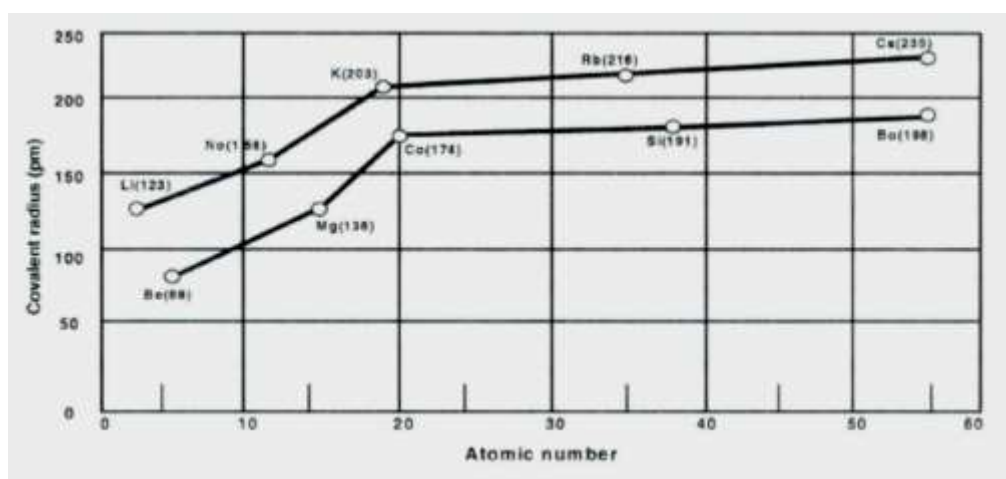
Fig. 4.3 Increase in Atomic Radii of Alkali and Alkaline Earth Metals Downward the Group
