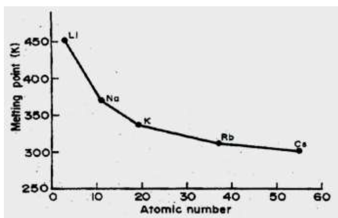
Fig. 2.3 Trend in the Melting Point of Group 1 Elements
