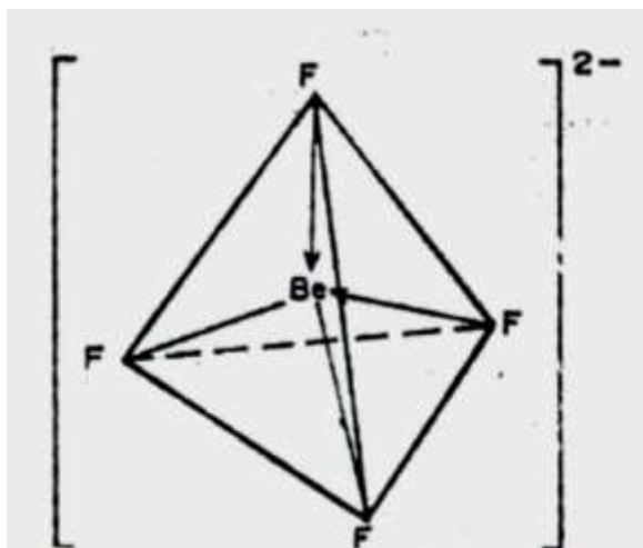
Fig. 2.2 Tetrafluoroberyllate Complex Ion (\text{BeF}_4)^{2-}
