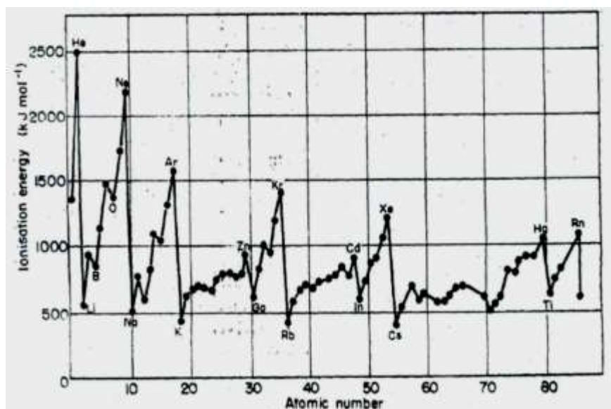
Fig. 5.1 The Plot of First Ionisation Energies of the Elements of the First Six Periods against their Atomic Numbers
