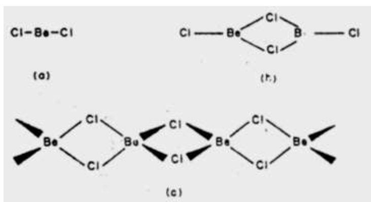
Fig. 1.4 Beryllium Chloride (a) Monomer (b) Dimer and (c) Polymer
