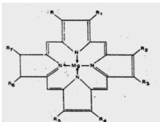
Fig. 2.4 Skeleton of Chlorophyll II Molecule
