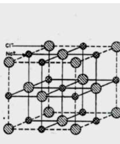
Fig. 1.3 Rock Salt ( \text{NaCl} ) Structure
