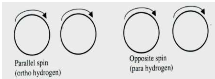
Fig. 3.2 Ortho and Para Forms of Hydrogen
