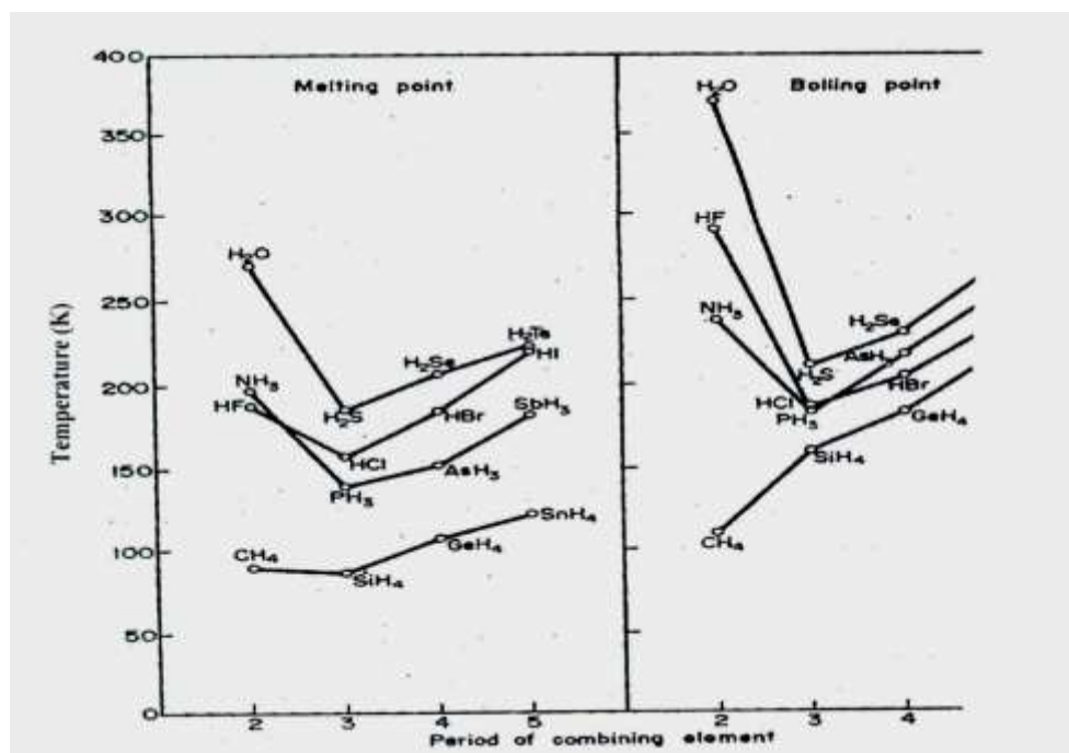
Fig. 1.1: (a) Melting point curves and (b) Boiling point curves of the molecular hydride
