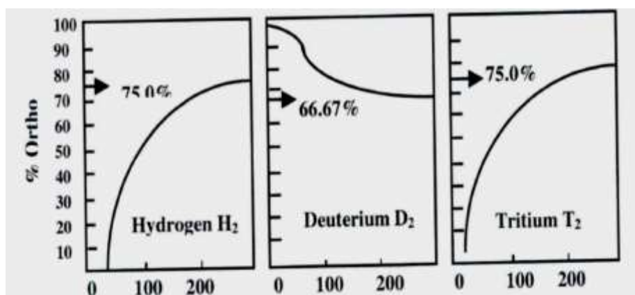
Fig. 3.3 Ortho-Para Equilibria for H 2 , D 2 and T 2
